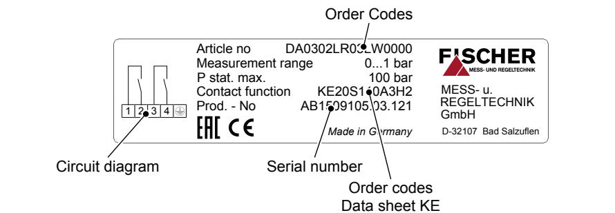
Fig. 3: Nameplate
