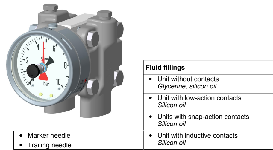
Fig. 5: Special functions
