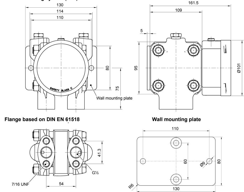
Fig. 23: Dimensional drawing (Small measuring system Ø75)
