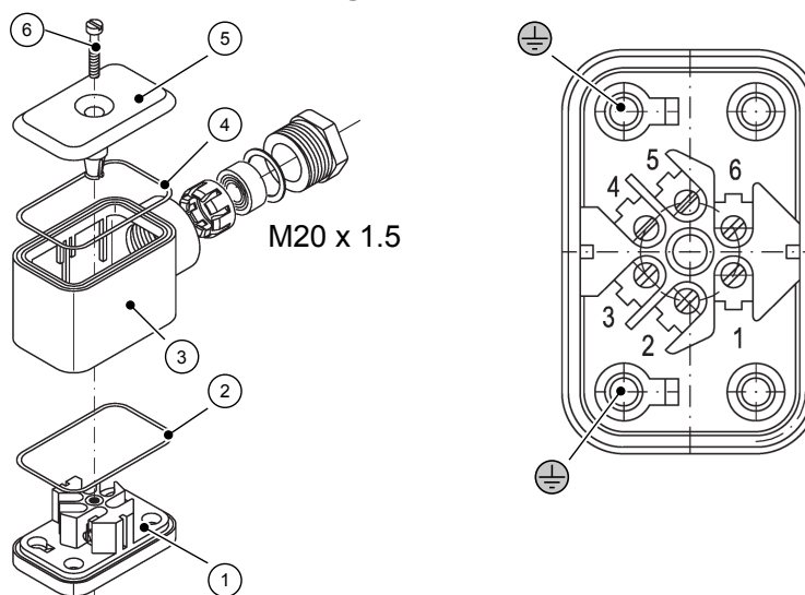
Fig. 13: Cable socket
