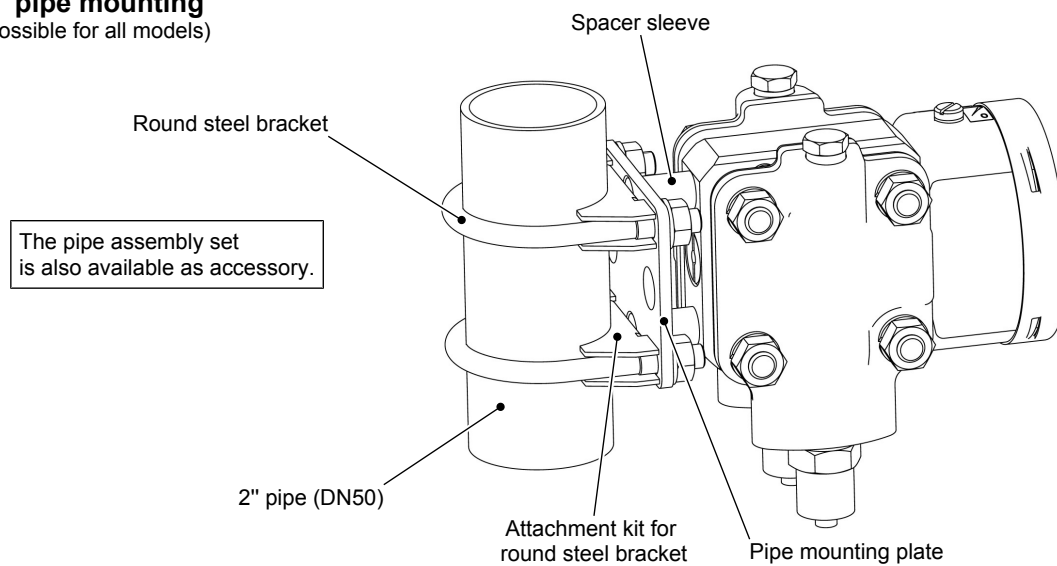
Fig. 13: Pipe mounting
