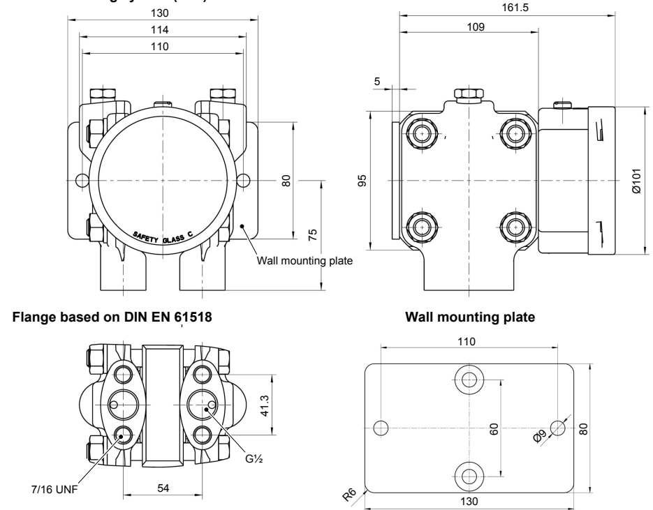
Fig. 12: Dimensional drawing (Small measuring system Ø75)
