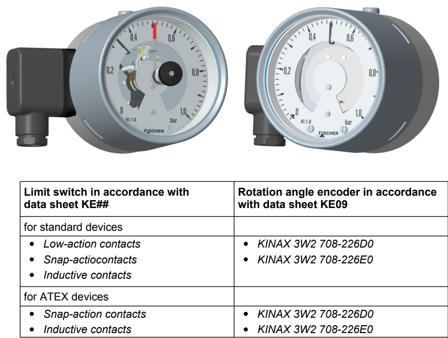
Fig. 3: Contact elements
