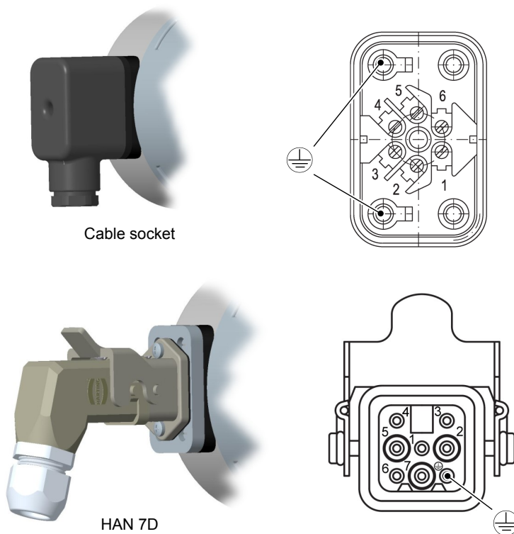
Fig. 11: Cable socket
