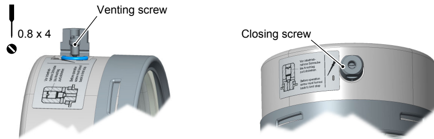
Fig. 15: Venting valve
