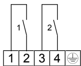
Fig. 12: Contacts
