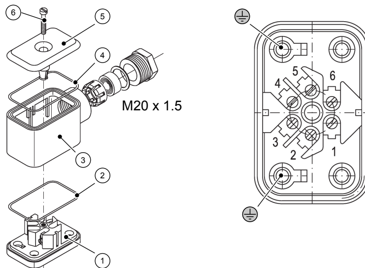
Fig. 10: Cable socket
