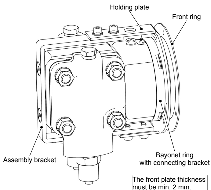
Fig. 23: Installation of front panel with panel fittings
