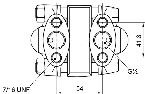
Fig. 20: Dimensional drawing (Small measuring system Ø75)
