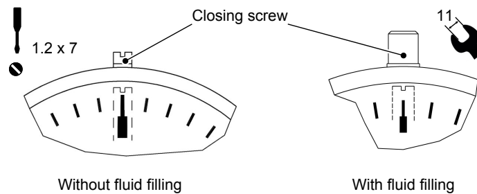
Fig. 17: Zero point correction screw
