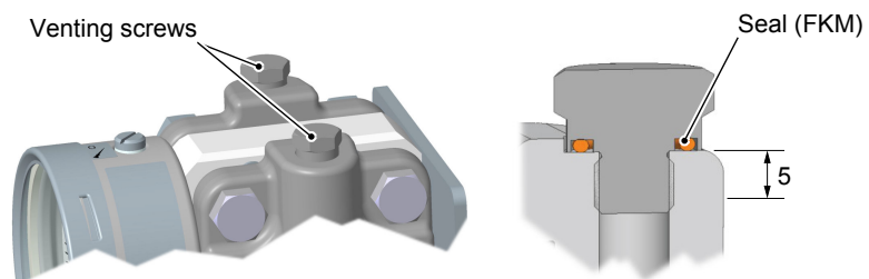
Fig. 16: Venting with fluid media
