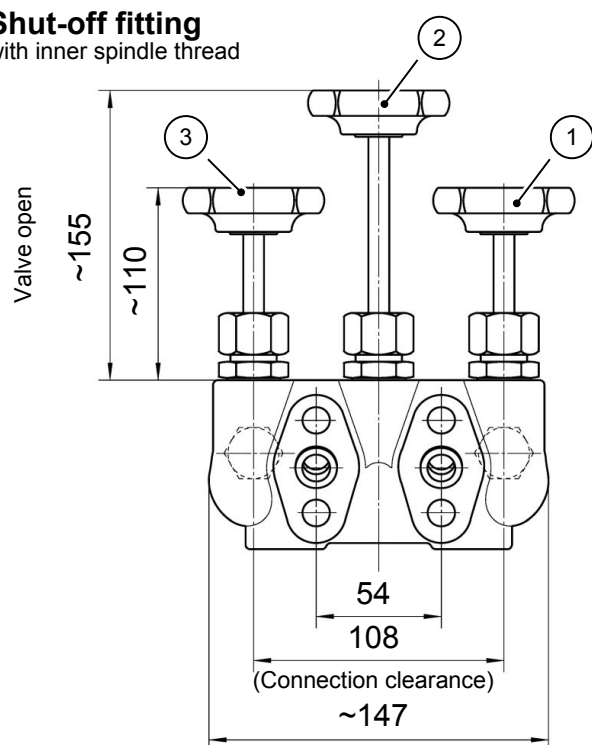
Fig. 26: Shutoff valve DZ3600SV2700
