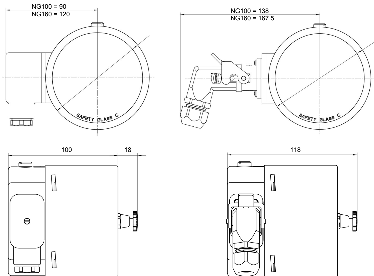
Fig. 25: Dimensional drawing contact devices
