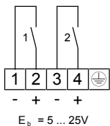
Fig. 13: Inductive contacts
