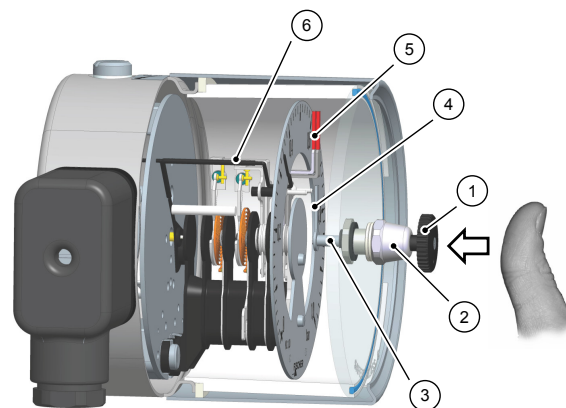
Fig. 18: Switch point setting
