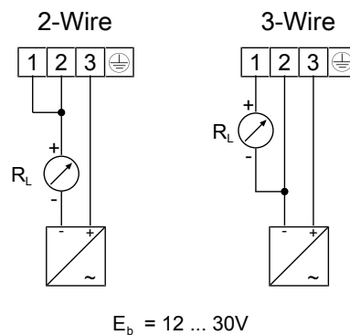
Fig. 14: Rotation angle transducers connection
