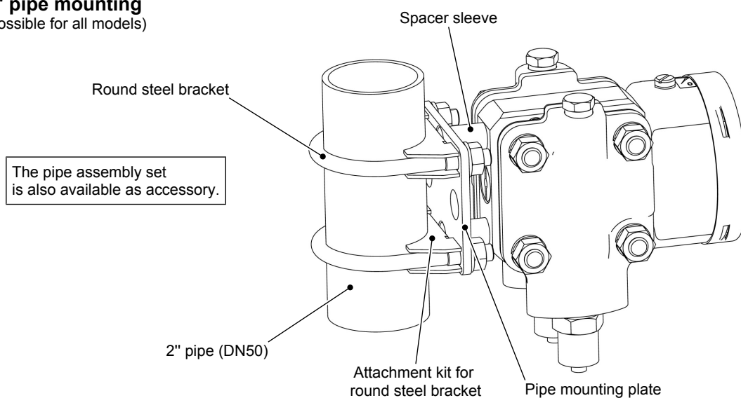
Fig. 21: Pipe mounting
