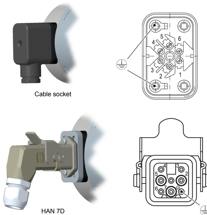
Fig. 19: Cable socket
