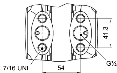
Fig. 22: Dimensional drawing (Large measuring system Ø130)
