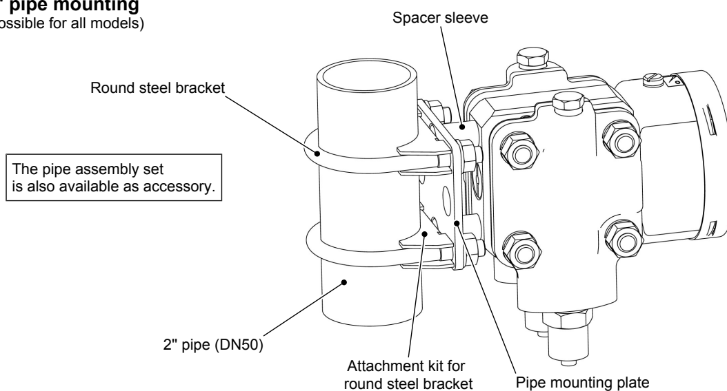
Fig. 9: Pipe mounting
